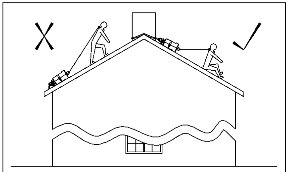
Figure 5 – Anchorage to minimise Fall Distance.
