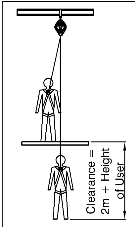
Figure 1. – Clearance Below
